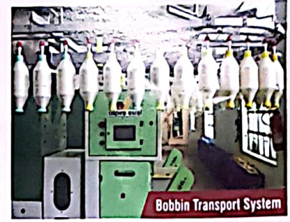
Auto Doffer Retrofit
